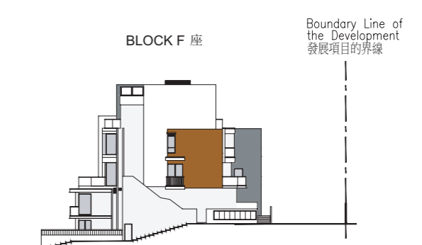
Elevation Plan V 立面圖V
