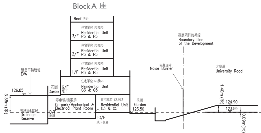
Cross-Section Plan A2 橫截面圖 A2
